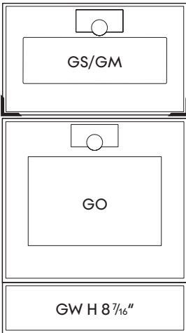
Combination EV3_21_H45_RNA (For dimensions, see page 10)
