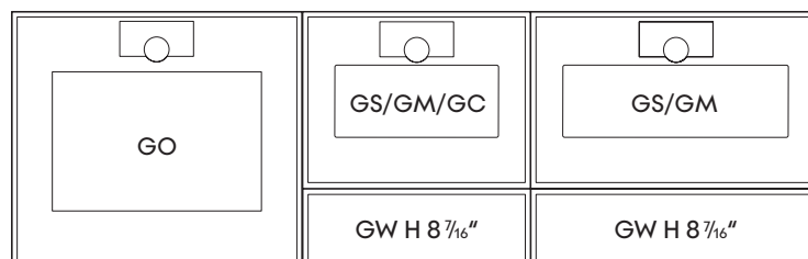
Combination EH363_21_RNA (For dimensions, see page 8)
