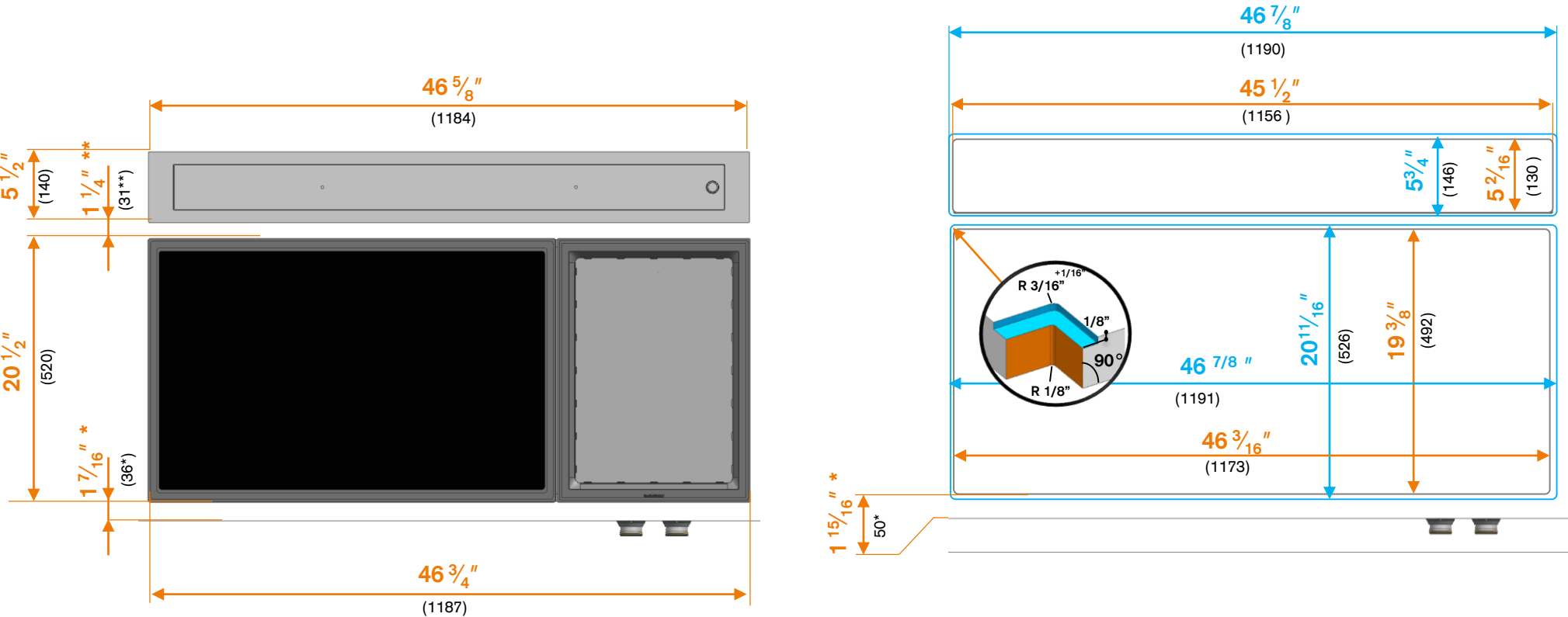
Cut out dimension. Flush mounting
