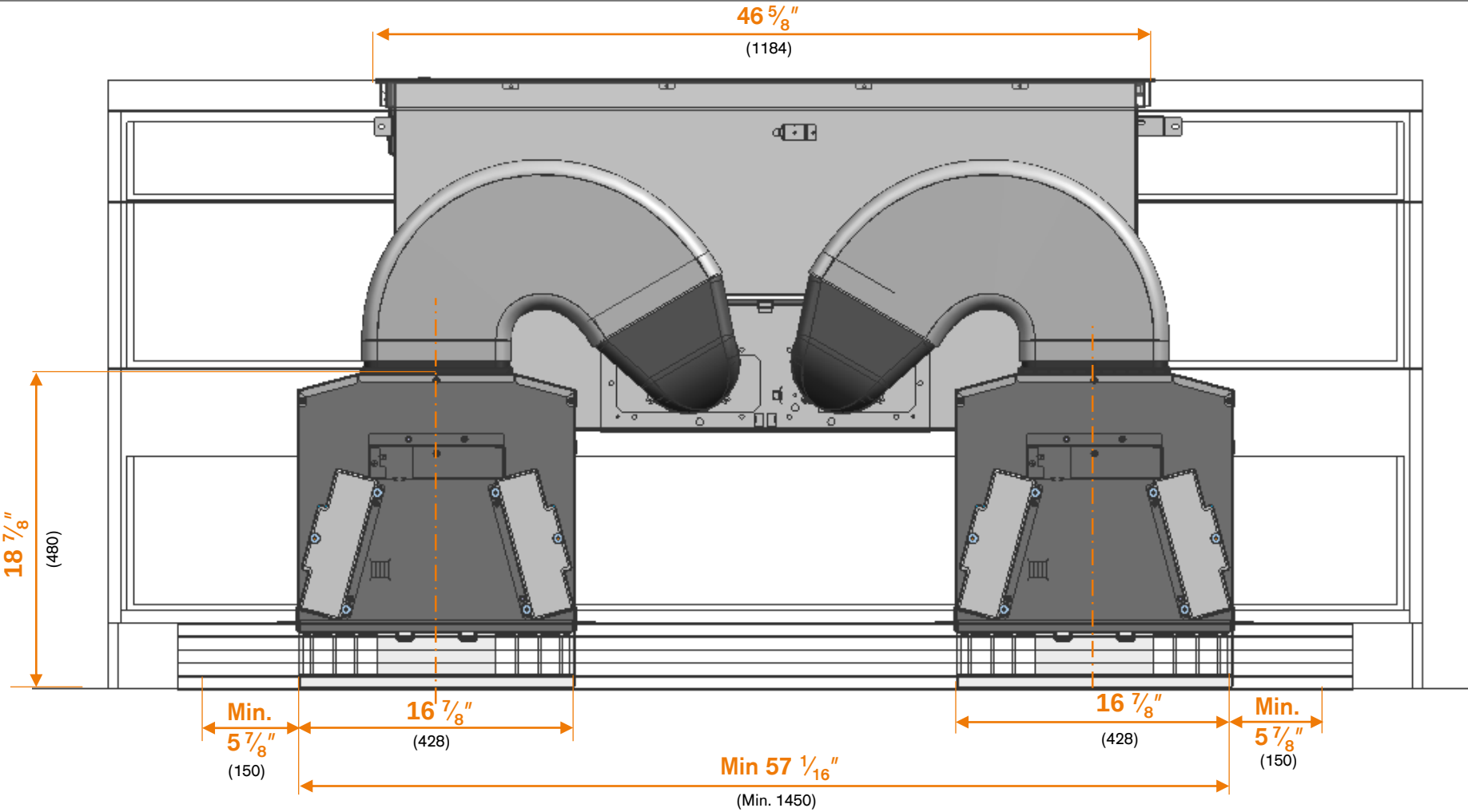
Back View
