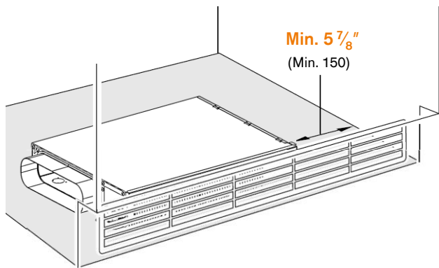
Min. distance for air outlet
