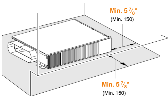
Min. distance for air outlet
