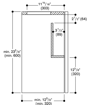
Cross-section of upper cabinet with AA 210 812 recirculation kit
