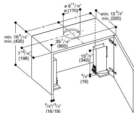
AA 210 812 recirculation kit
