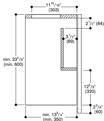
Cross-section of upper cabinet with AA 210 812 recirculation kit
