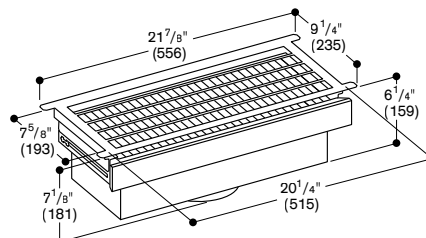
AA 210 812 recirculation kit
