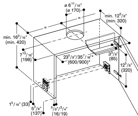
Upper cabinet for 24"/36" AF visor hood
