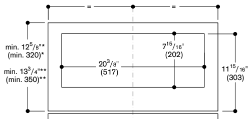
View from above of upper cabinet with AA 210 812 recirculation kit
