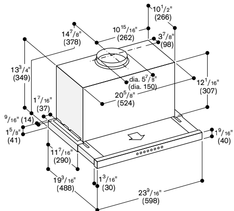
Measurement drawing of 24" AF visor hood
